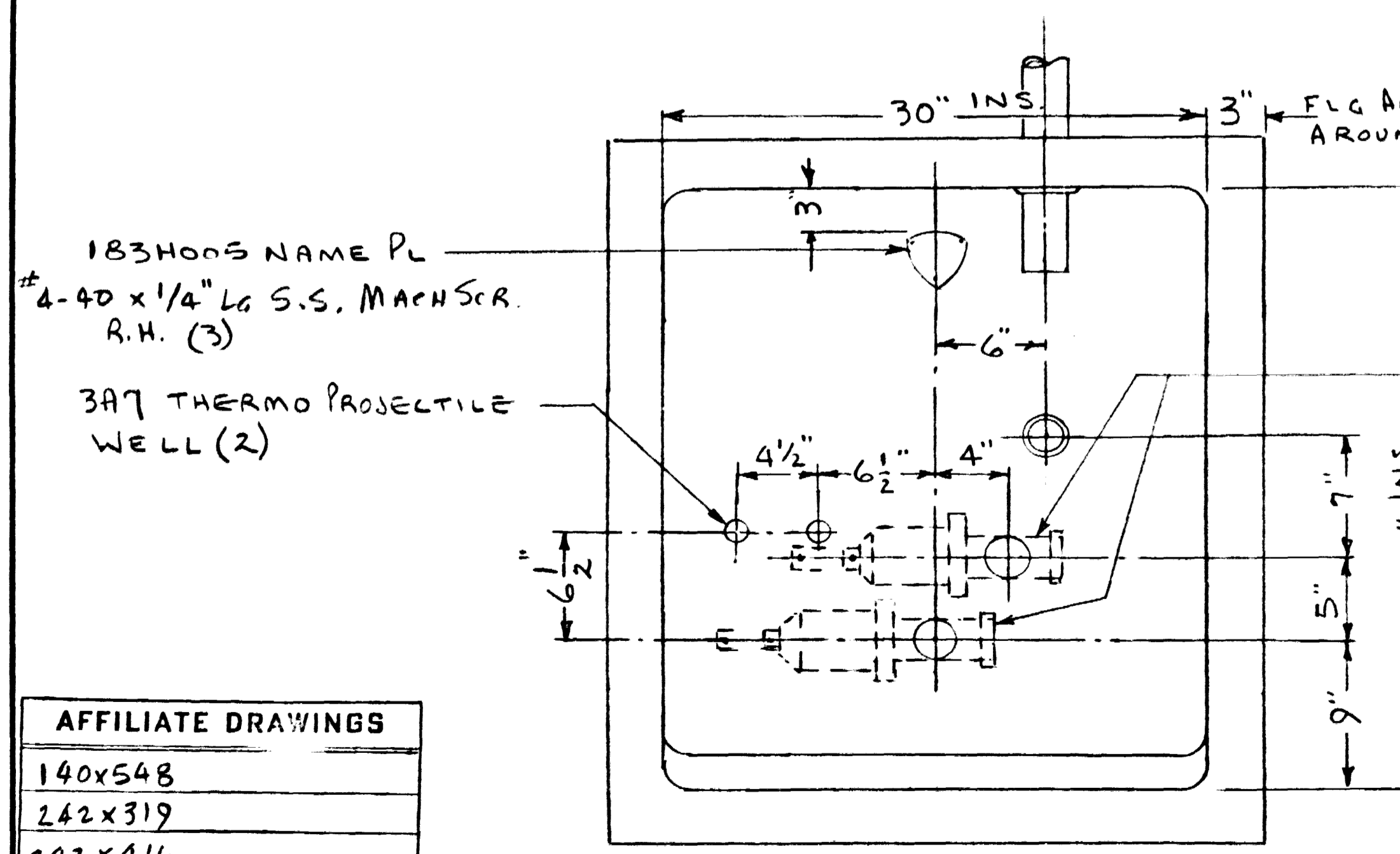
ALCOVE LAYOUT - 1/8 SCALE
