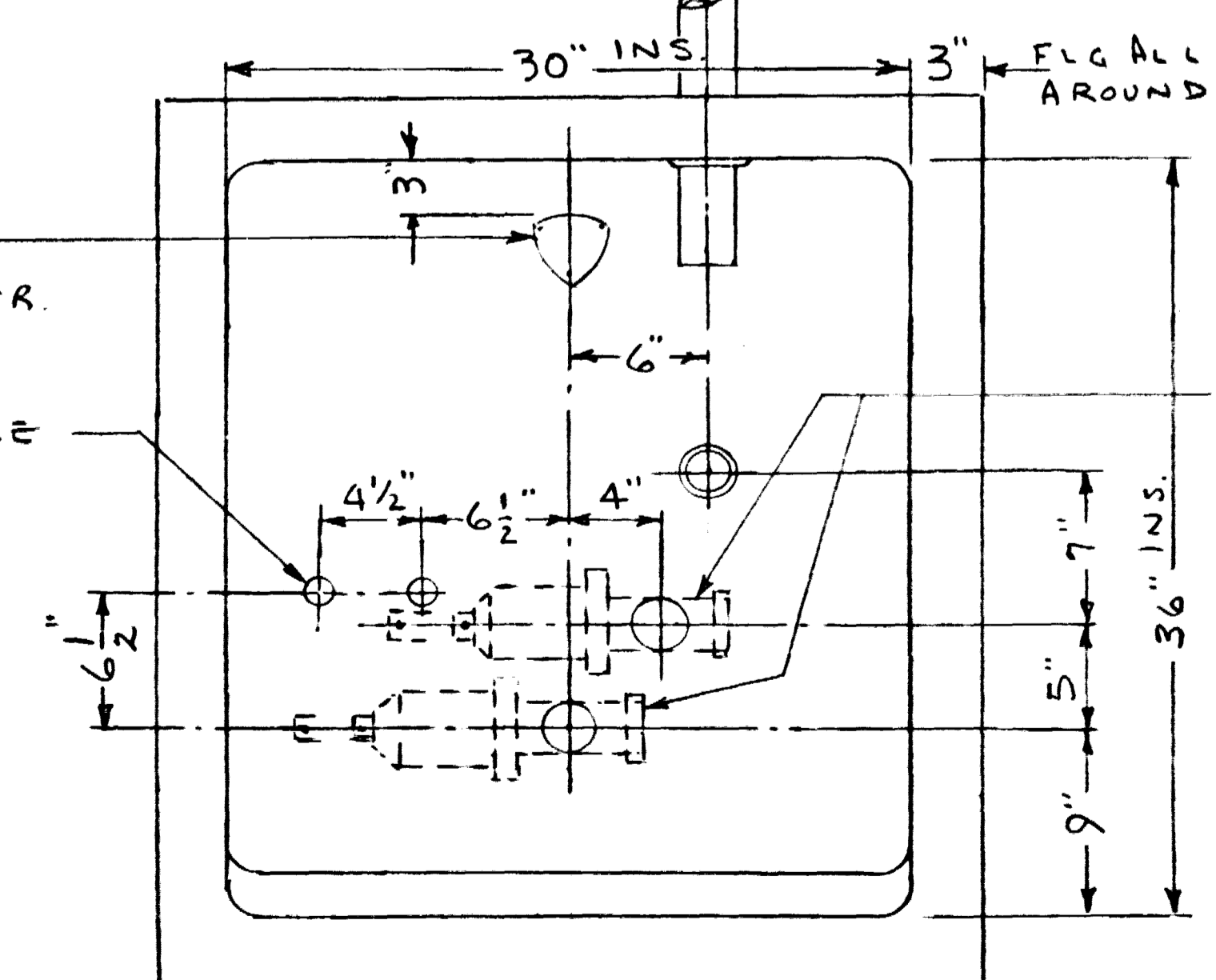
ALCOVE LAYOUT - 1/8 SCALE
